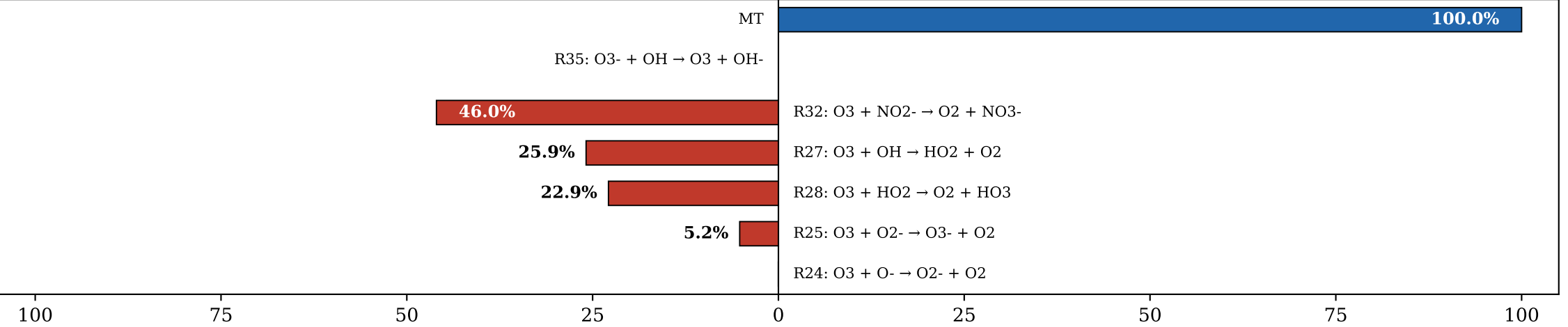
(c) NO 2 - (Σsrc = 3.13e-08 M/s)
