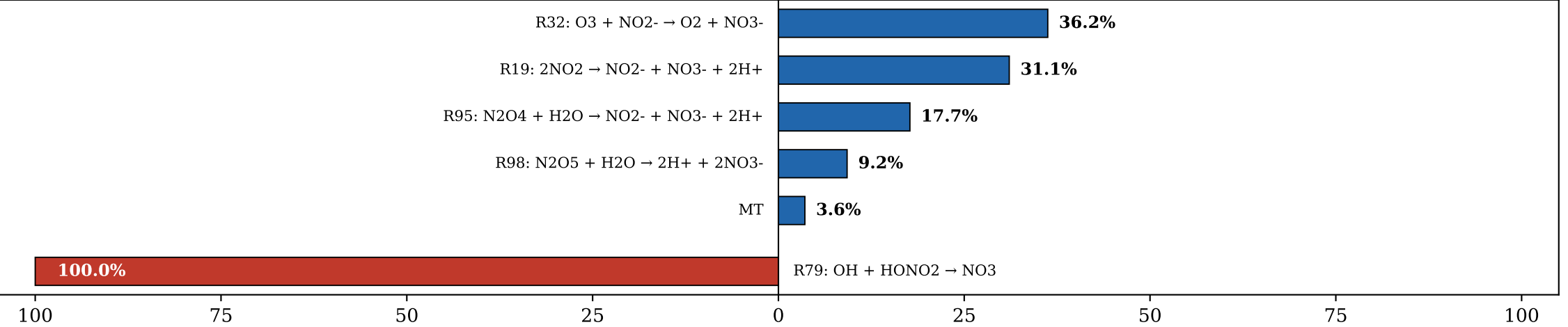
(b) O 3 (Σsrc = 5.85e-08 M/s)
